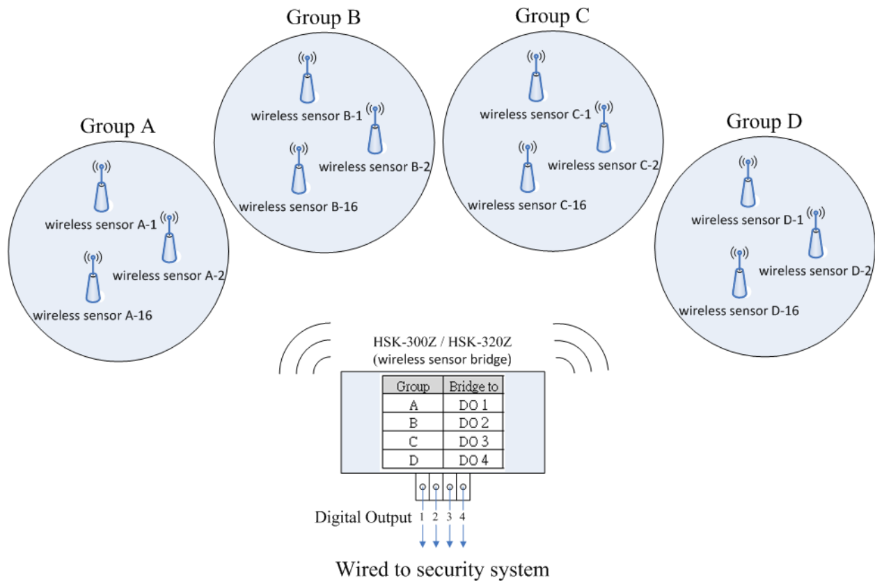
Wireless sensor bridge Schematic diagram
